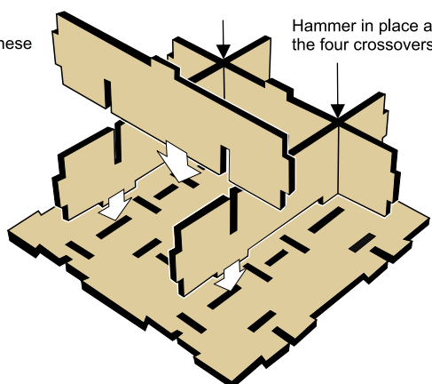
Side pieces
